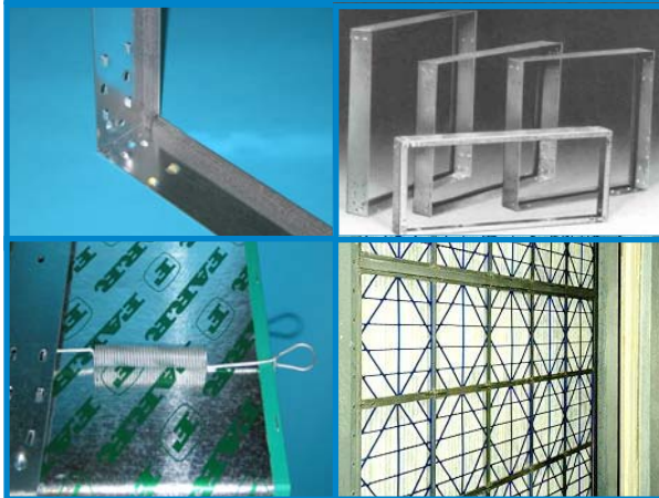
Top: Type 8 corner showing centering dimples, lances, welded construction and filter sealing gasket
